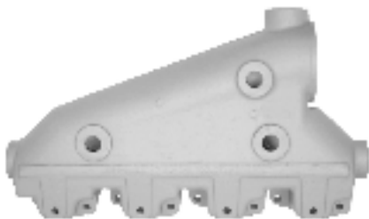
18-1933 Manifold Crusader GM Big Block V8 454cu.in. (Models: CH350 and 454XL) Replaces: Crusader 97993 & 97115
